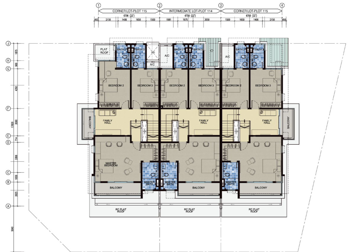
TYPE A ( 22' X 75' DSTH ) FIRST FLOOR PLAN
